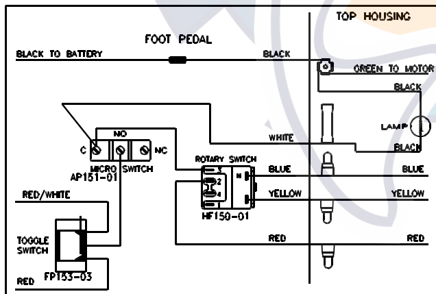
12/24 WIRING DIAGRAM
